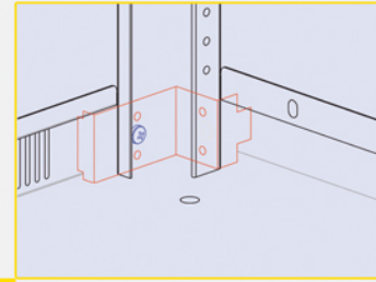
8 Welded Corner Bracket Mounting
