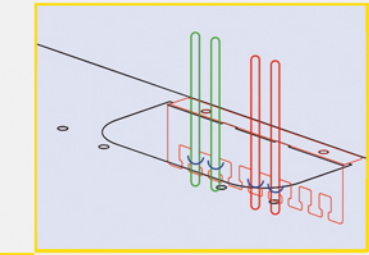
12 Cabling Details
