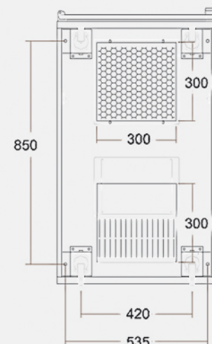
Bottom Panel Details
