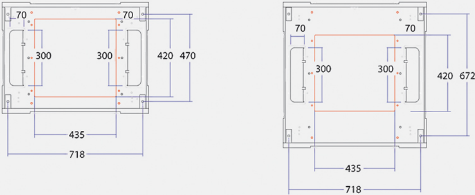
Section-A Details Dimensions in mm
