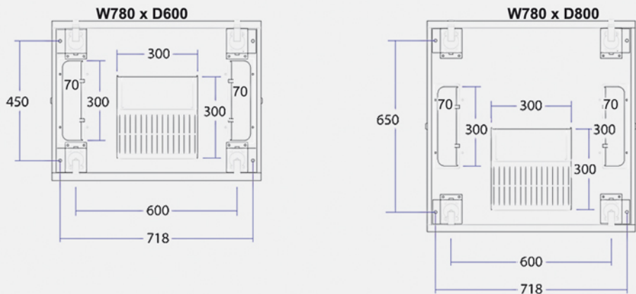
Bottom Panel Details Dimensions in mm
