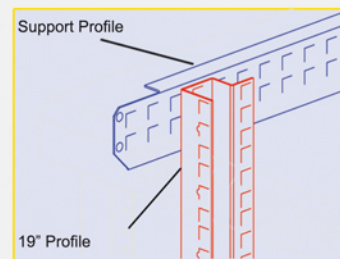
9 Support Profile Mounting
