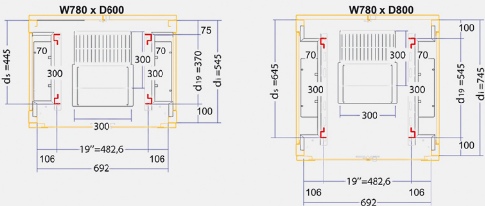
Bottom Panel Details Dimensions in mm
